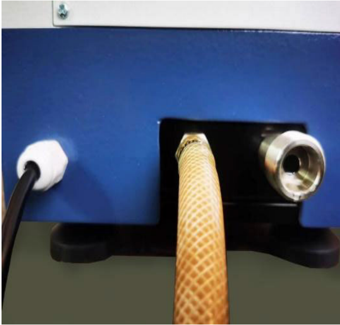
Water Inlet/Outlet
